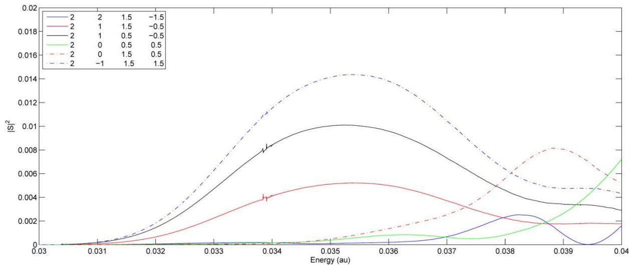
Figure 47. Probability to Transition from \begin{vmatrix} 0 & \frac{1}{2} \\ 0 & \frac{1}{2} \end{vmatrix}, 0 to the Six Allowed \begin{vmatrix} 2 & J_a \\ j & \omega \end{vmatrix}, 1 States
