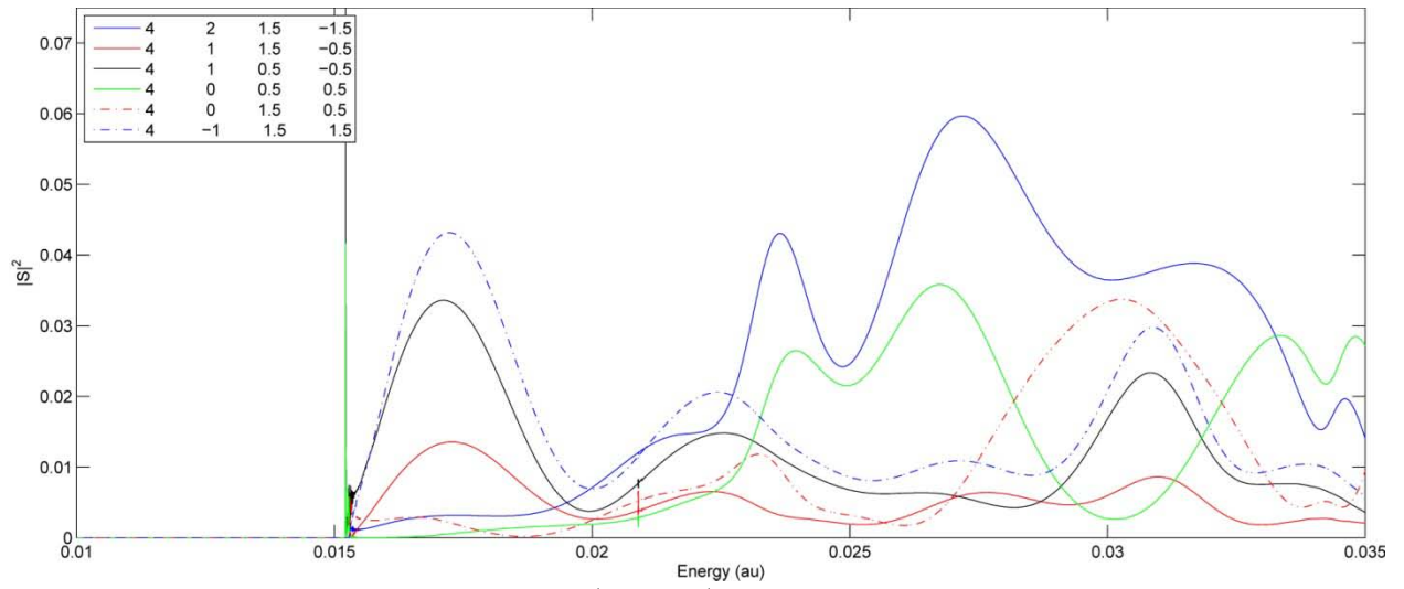
Figure 38. Probability to Transition from \left| \begin{matrix} 0 & \frac{1}{2} \\ 0 & \frac{1}{2} \end{matrix}, 0 \right\rangle to the Six Allowed \left| \begin{matrix} 4 & j_a \\ j & \omega \end{matrix}, 0 \right\rangle States
