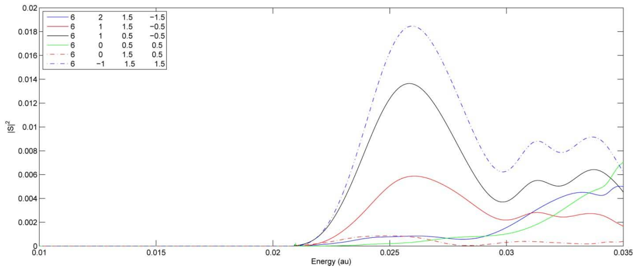
Figure 39. Probability to Transition from \left| \begin{matrix} 0 & \frac{1}{2} \\ 0 & \frac{1}{2} \end{matrix}, 0 \right\rangle to the Six Allowed \left| \begin{matrix} 6 & j_a \\ j & \omega \end{matrix}, 0 \right\rangle States
