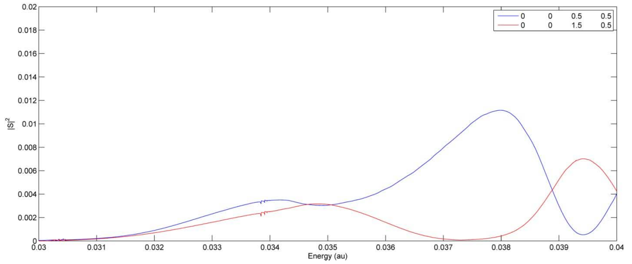
Figure 46. Probability to Transition from \begin{vmatrix} 0 & \frac{1}{2} \\ 0 & \frac{1}{2} \end{vmatrix}, 0 to \begin{vmatrix} 0 & \frac{1}{2} \\ 0 & \frac{1}{2} \end{vmatrix}, 1 and \begin{vmatrix} 0 & \frac{3}{2} \\ 0 & \frac{1}{2} \end{vmatrix}, 1
