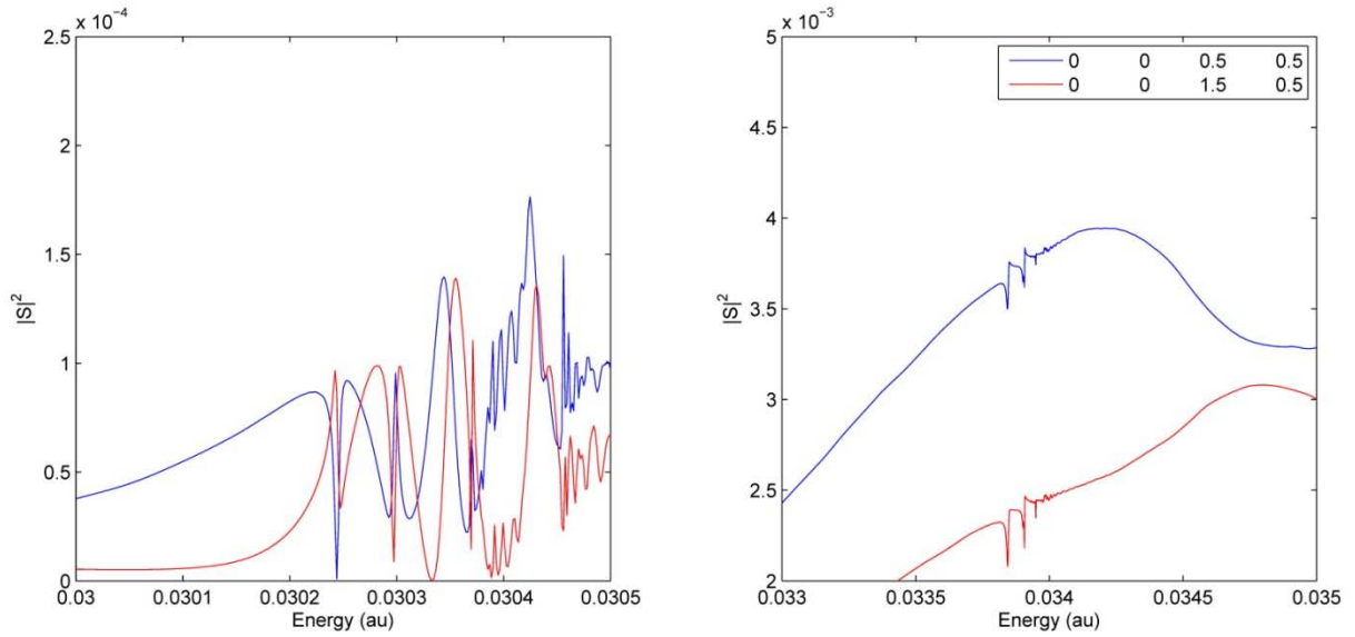
Figure 52. Feshbach Resonance Detail for Transition from \begin{pmatrix} 0 & \frac{1}{2} \\ 0 & \frac{1}{2} \end{pmatrix}, 0 to \begin{pmatrix} 0 & \frac{1}{2} \\ 0 & \frac{1}{2} \end{pmatrix}, 1 and \begin{pmatrix} 0 & \frac{3}{2} \\ 0 & \frac{1}{2} \end{pmatrix}, 1
