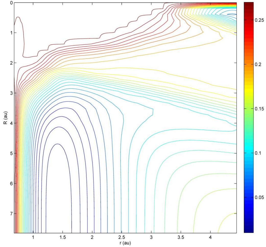
Figure 8. Diabatic Effective Potential Energy Surface \left\langle 2, \frac{3}{2} \left| V_{eff}^D(r, R) \right| 2, \frac{3}{2} \right\rangle Contour Plot
