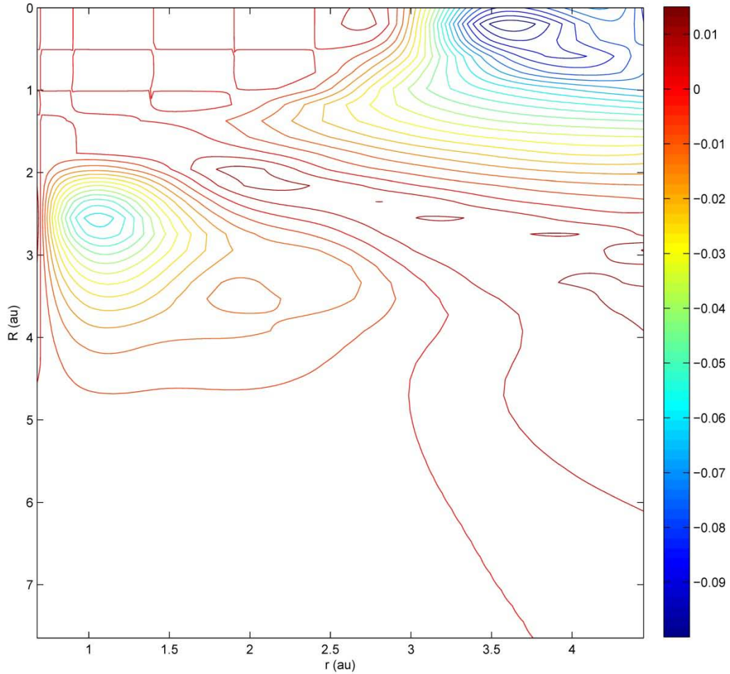
Figure 10. The Coupling Surface \left\langle 0, \frac{1}{2} \left| V_{eff}^D(r, R) \right| 0, \frac{3}{2} \right\rangle Contour Plot
