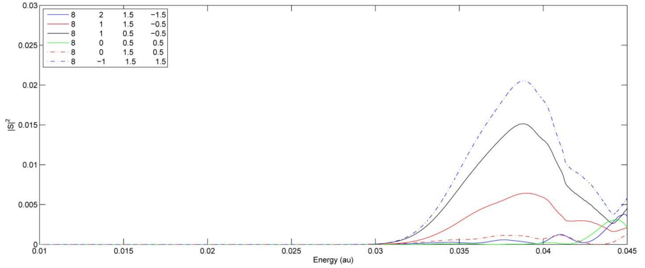
Figure 40. Probability to Transition from \left| 0 \begin{array}{c} \frac{1}{2} \\ \frac{1}{2} \end{array}, 0 \right\rangle to the Six Allowed \left| \begin{array}{c} 8 \\ j \end{array} \begin{array}{c} j_a \\ \omega \end{array}, 0 \right\rangle States
