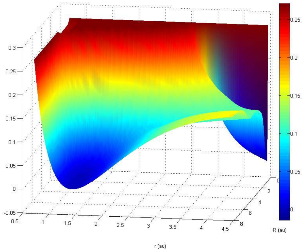
Figure 5. Diabatic Effective Potential Energy Surface \left\langle 0, \frac{1}{2} \left| V_{eff}^D(r, R) \right| 0, \frac{1}{2} \right\rangle
