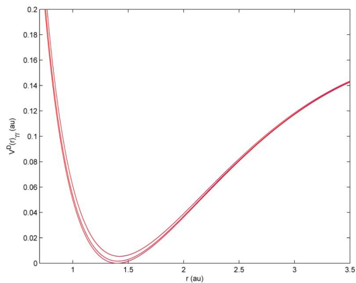
Figure 21. Cross-sections of the Diabatic PESs for j = 0, 2, 4 at Limit of Large R
