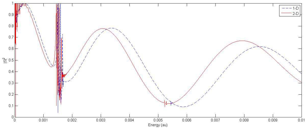
Figure 55. 1-D and 2-D Results for the Transition from \left| \begin{smallmatrix} 0 & \frac{1}{2} \\ 0 & \frac{1}{2} \end{smallmatrix}, 0 \right\rangle to \left| \begin{smallmatrix} 0 & \frac{1}{2} \\ 0 & \frac{1}{2} \end{smallmatrix}, 0 \right\rangle
