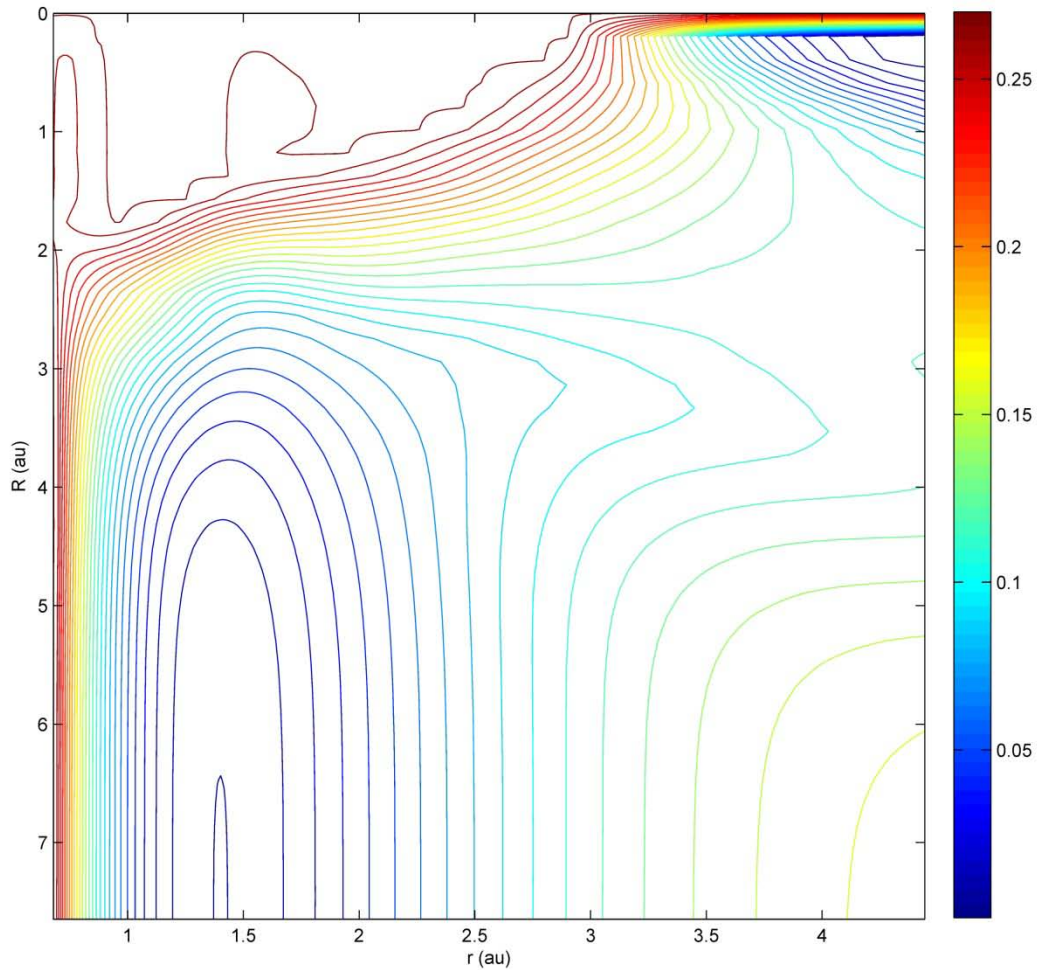
Figure 6. Diabatic Effective Potential Energy Surface \left\langle 0, \frac{1}{2} \left| V_{eff}^D(r, R) \right| 0, \frac{1}{2} \right\rangle Contour Plot
