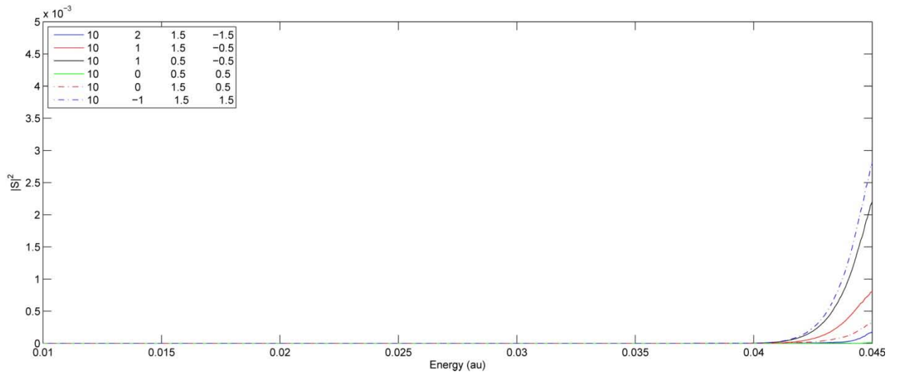
Figure 41. Probability to Transition from \left| 0 \begin{array}{c} \frac{1}{2} \\ \frac{1}{2} \end{array}, 0 \right\rangle to the Six Allowed \left| \begin{array}{c} 10 \\ j \end{array} \begin{array}{c} j_a \\ \omega \end{array}, 0 \right\rangle States
